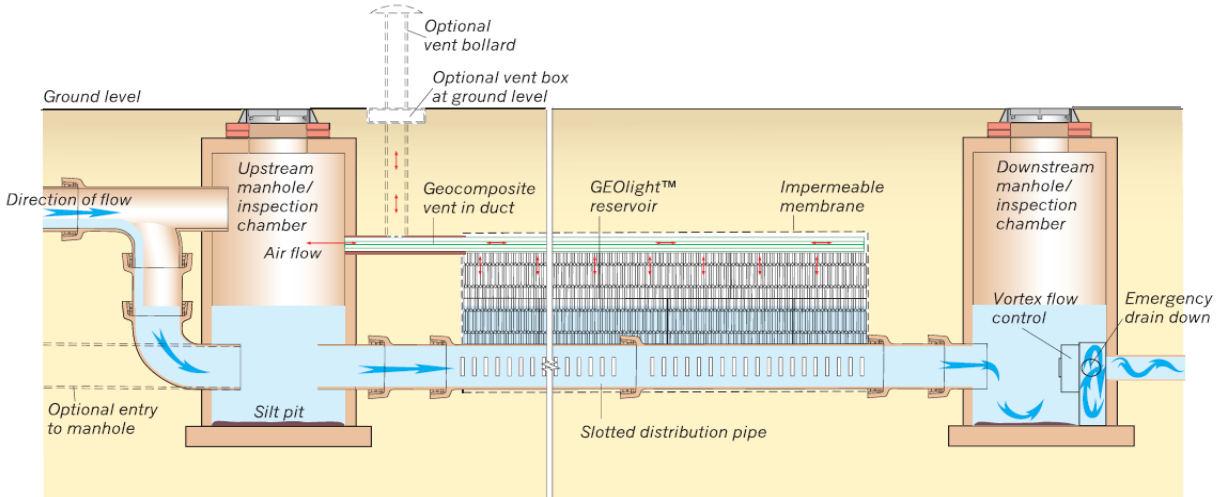
Figure DS 1.0: SDS Geolight cellular storage solution, which can be positioned below highways, or car parks if necessary.
