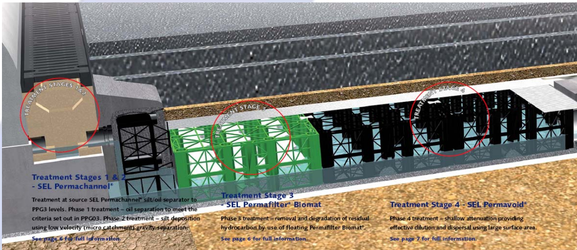
Figure DS 1.1: Althon SUDS car park cellular storage solution, which treats flows prior to discharge.
